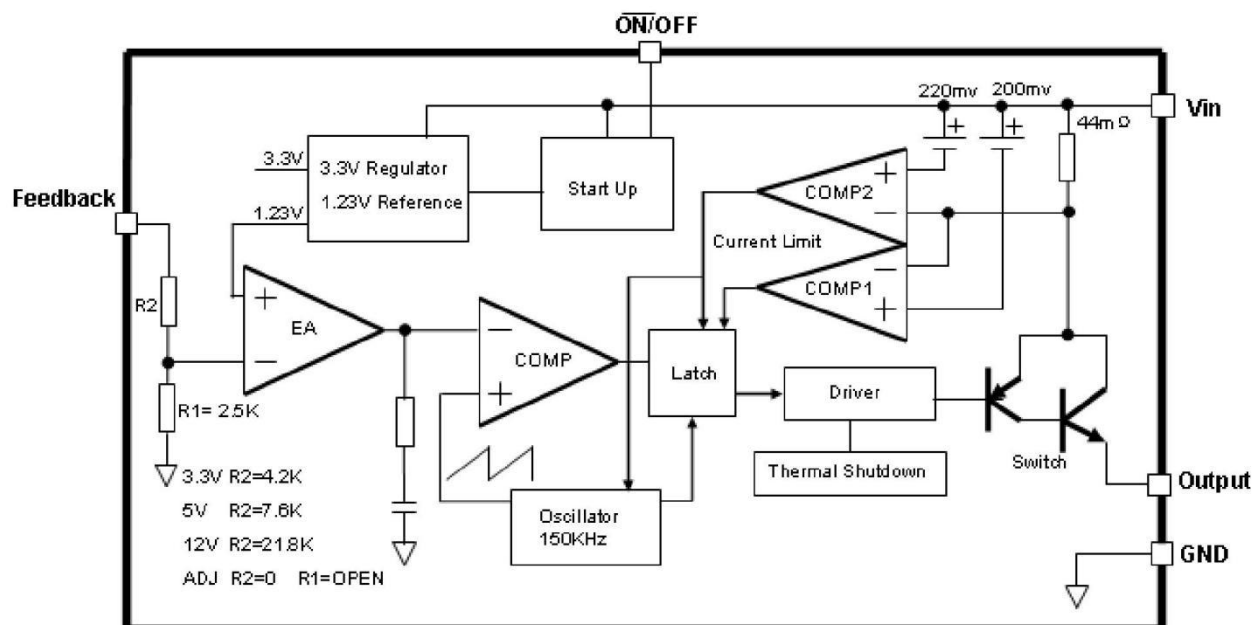
Figure3. Function Block Diagram of YCC1509
