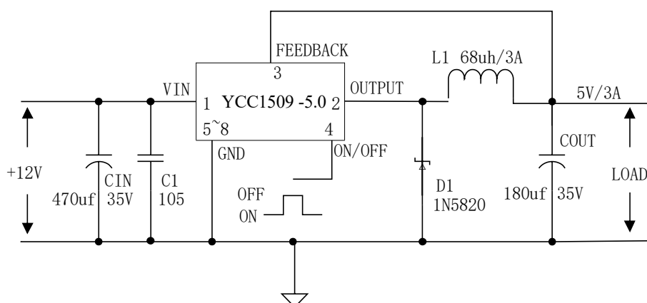
Figure4. YCC1509 Typical Application Circuit 12V-5V/3A
