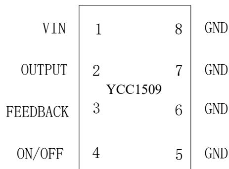
Figure2. Pin Configuration of YCC1509 (Top View)
