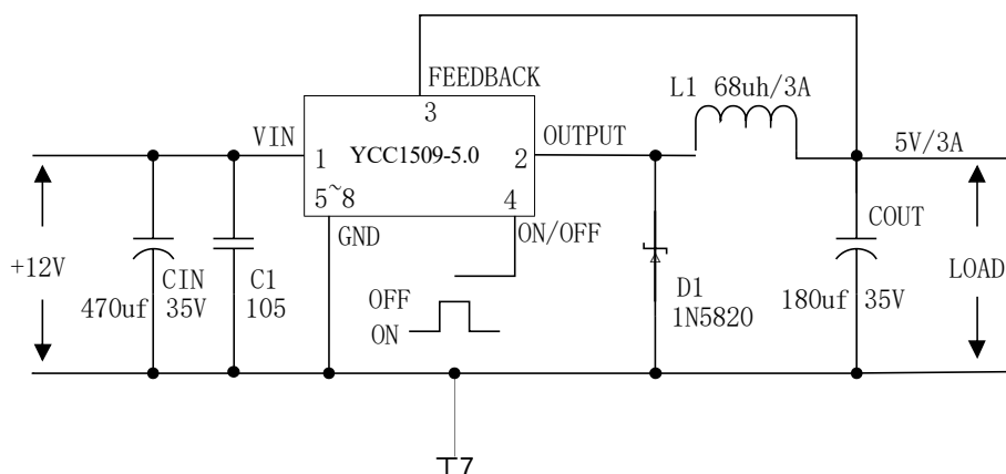
Figure7. YCC1509-5.0 System Parameters Test Circuit
