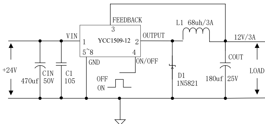
Figure8. YCC1509-12 System Parameters Test Circuit
