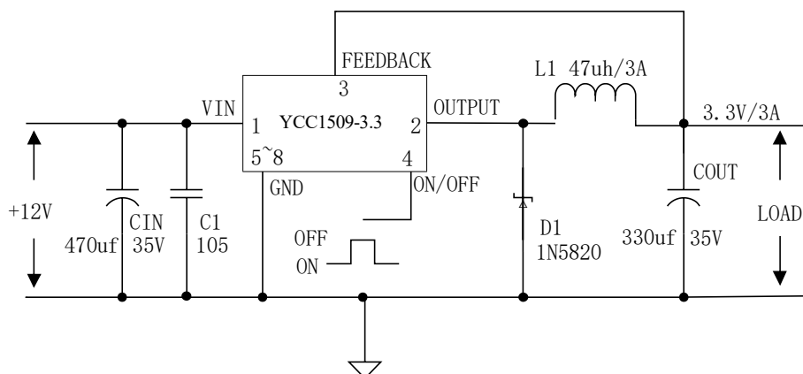
Figure6. YCC1509-3.3 System Parameters Test Circuit
