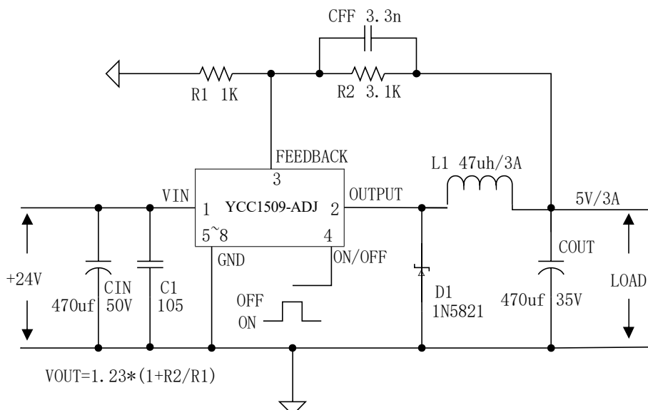
Figure9. YCC1509-ADJ System Parameters Test Circuit
